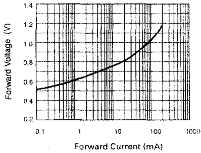
Forward Characteristics
