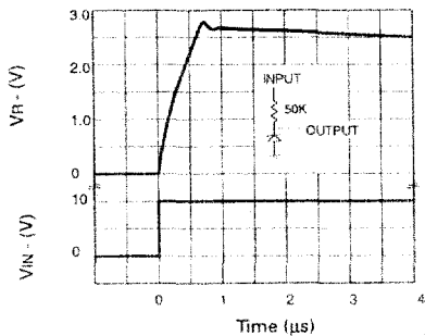
Transient Response ( I_R = 150\mu\text{A} )
